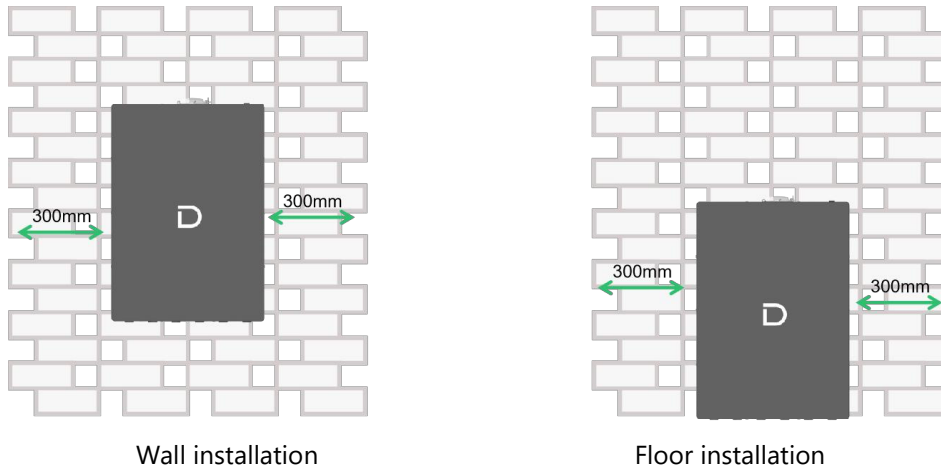
Figure 3-3 Mounting Space Requirements
