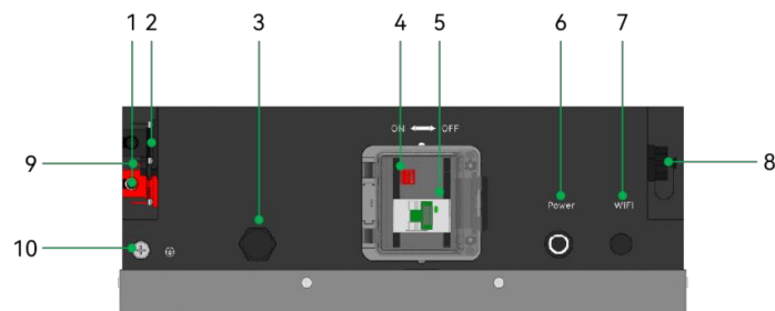
Figure 2-1 PowerHaus the Sketch of Front Interface
