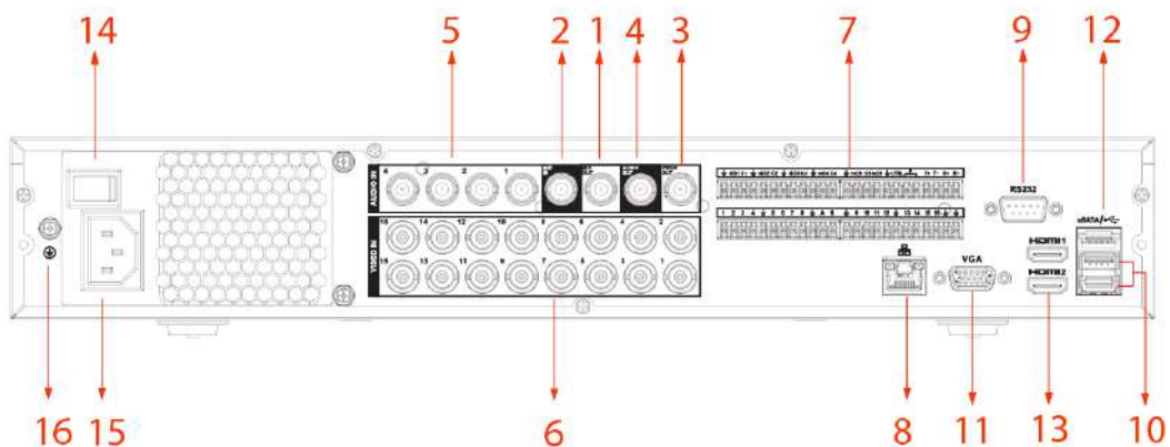
Figure 3-20 Rear panel (3)
