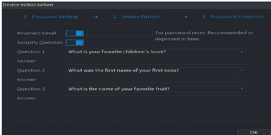
Figure 5-5 Password protection
