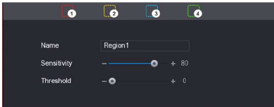
Figure 5-123 Detection setting
