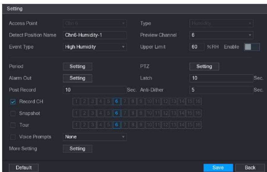
Figure 5-219 Setting
