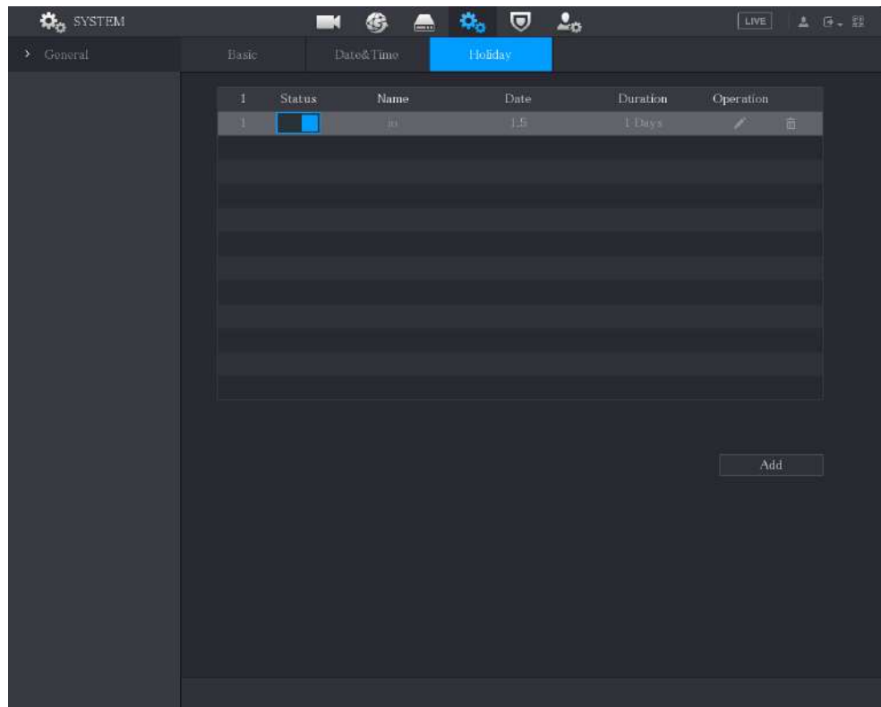
Figure 5-304 Added holiday
