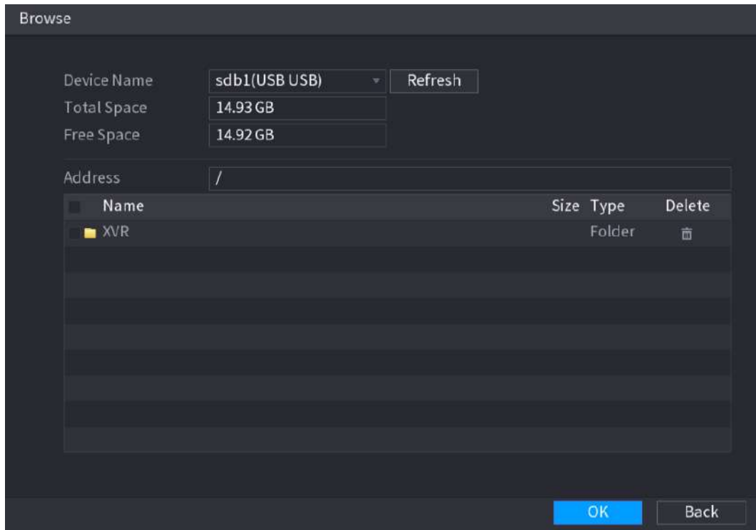
Figure 5-145 Browse
