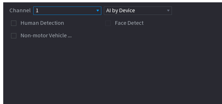
Figure 5-177 Video structuring
