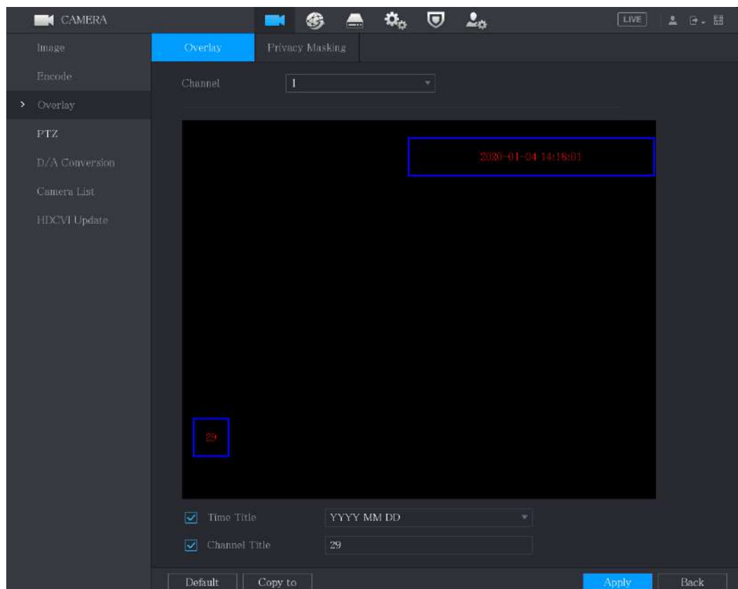
Figure 5-68 Overlay
