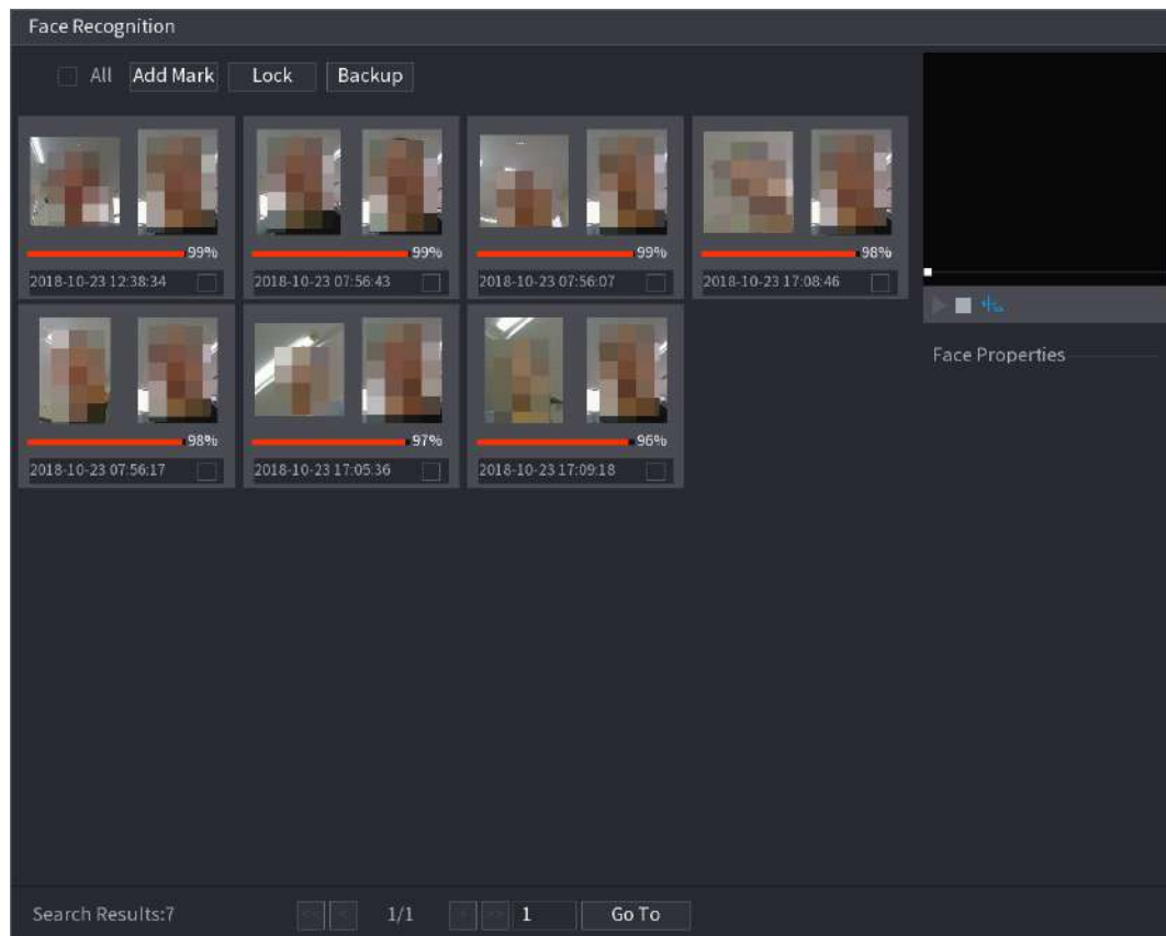
Figure 5-163 Search results
