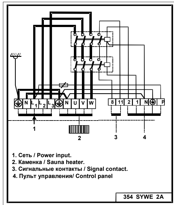
Contactor box
