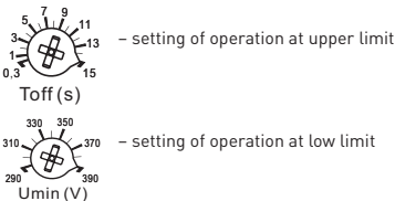
Pic. 2 Control panel
