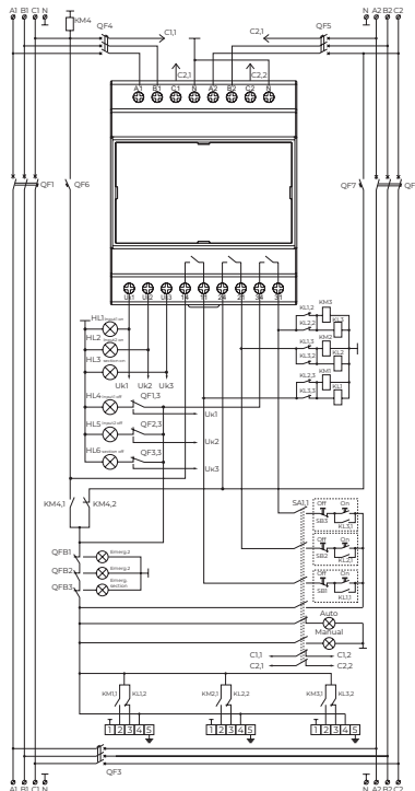
Pic. 5 Wiring diagram with circuit breakers and electric drives
