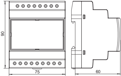
Pic. 1 Overall dimensions
