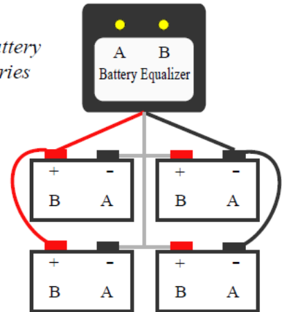
■ Figure 4: 48V battery bank
