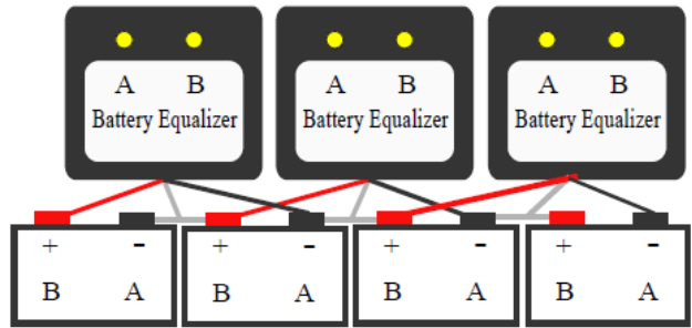
■ Figure 4: 48V battery bank
