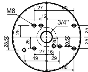
FLANGE DETAIL
