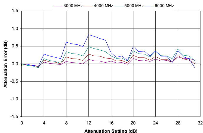
Figure 15. 1 dB Attenuation Error (continued)
