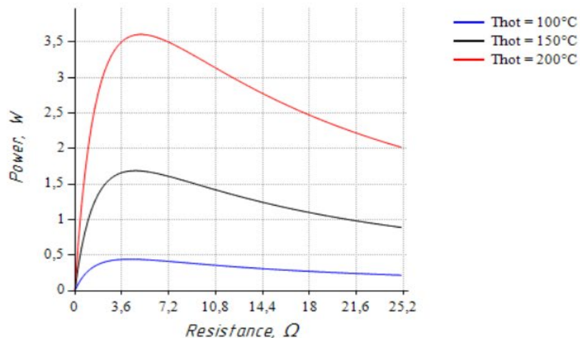
Output power vs. Load resistance (at T_{cold} = 50^\circ C )
