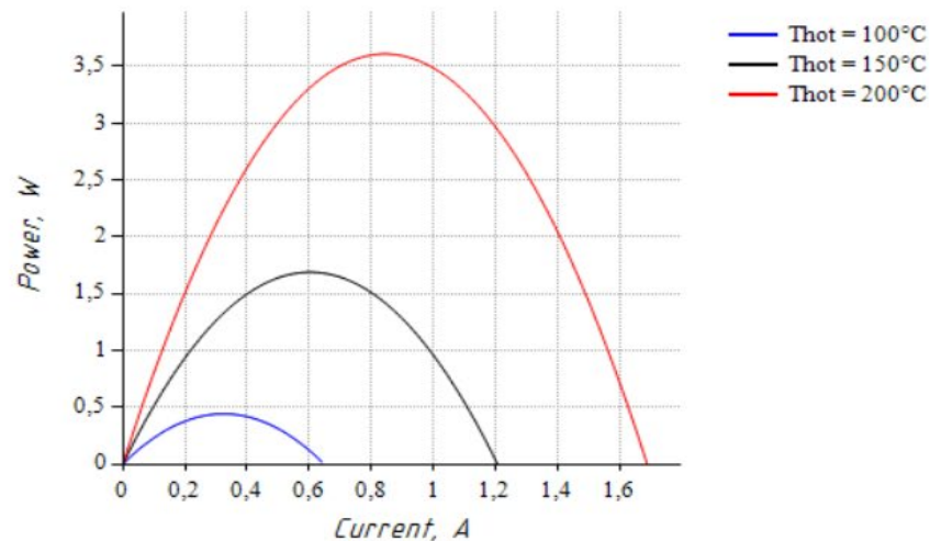
Output power vs. Current (at T_{cold} = 50^\circ C )
