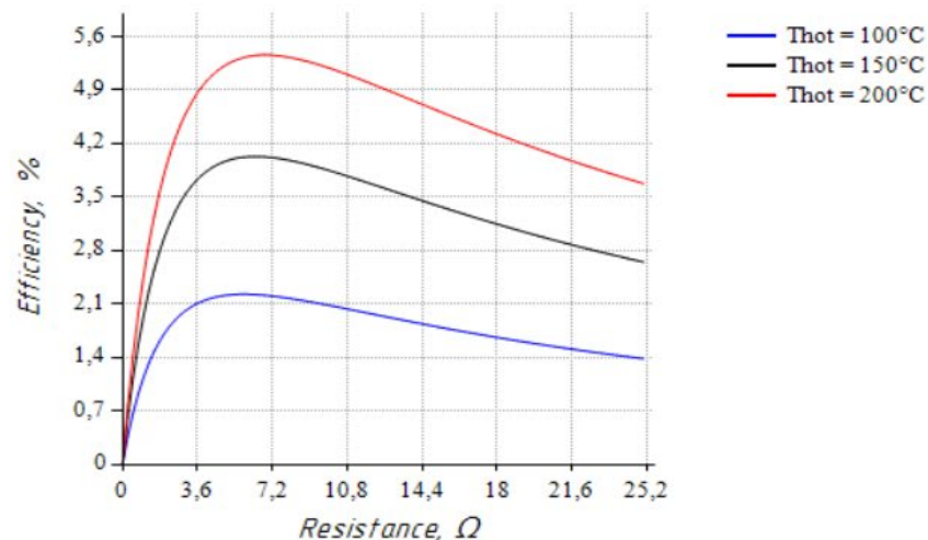
Efficiency vs. Load resistance (at T_{cold} = 50^\circ C )
