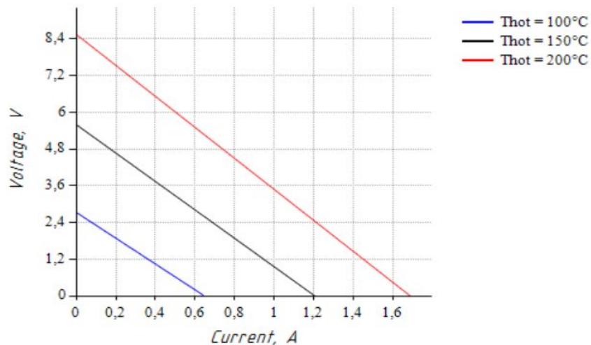
Voltage vs. Current (at T_{cold} = 50^\circ C )
