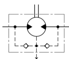
Figure 1 OMSU built-in check valves
