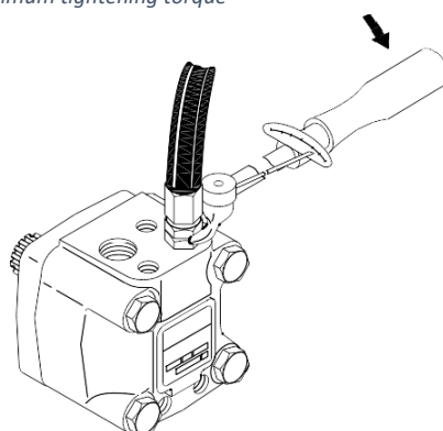
Figure 7 Tightening
