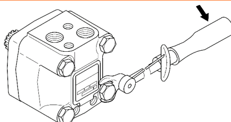
Figure 5 Mounting
