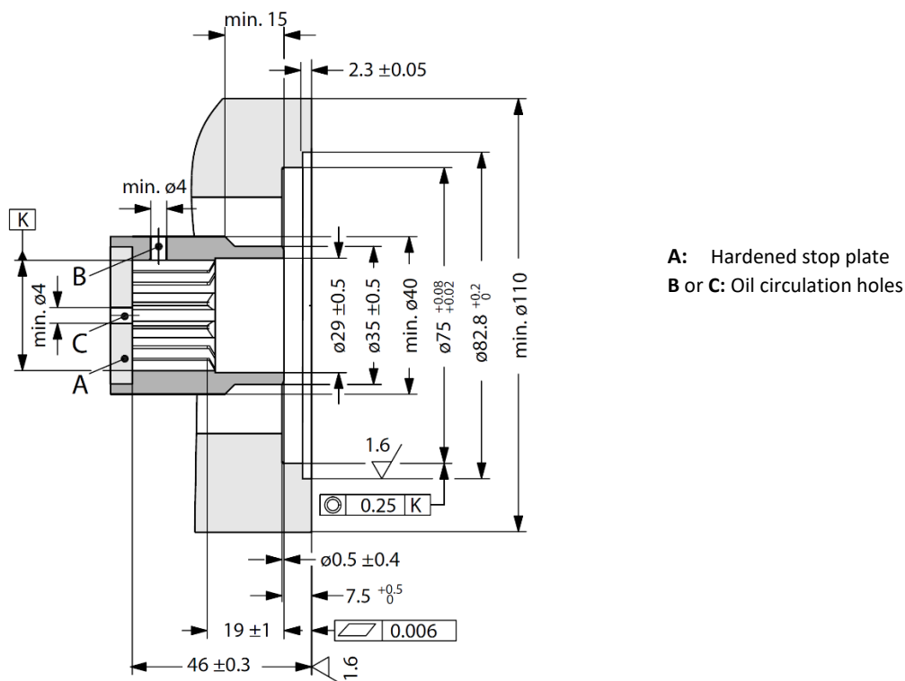
Figure 3 Connection dimensions
