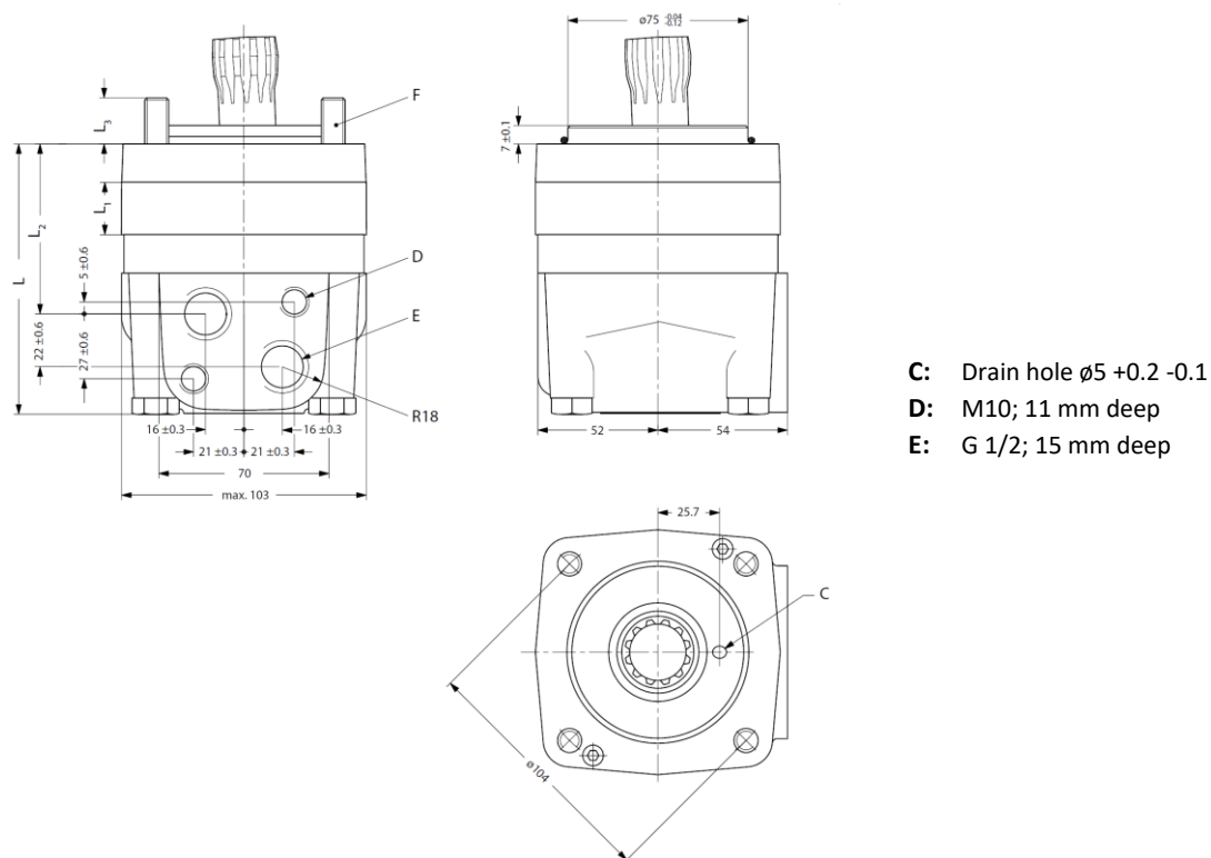
Figure 2 OMSU dimensions
