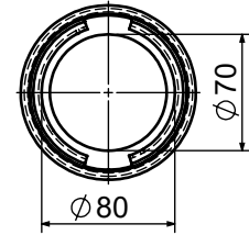
4-Dolum Boğazı / Filling Neck(Ø80mm)
