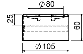
5-Şamandra / Level sensor
