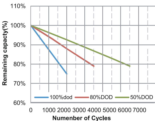
Different DOD Discharge Cycle Life Curve@0.5C, 25
