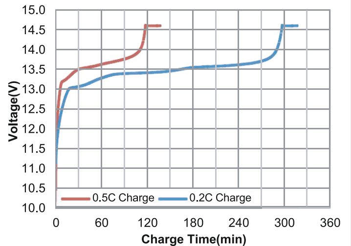
Charge Characteristics @0.2C&0.5C, 25°C
