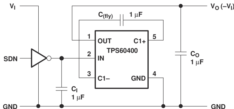
Figure 9-10. Shutdown Control
