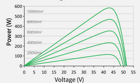
Power-Voltage (590W)
