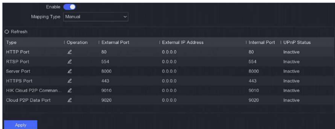
Figure 6-4 NAT
