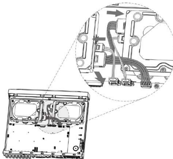
Figure 2-5 Connect cables
