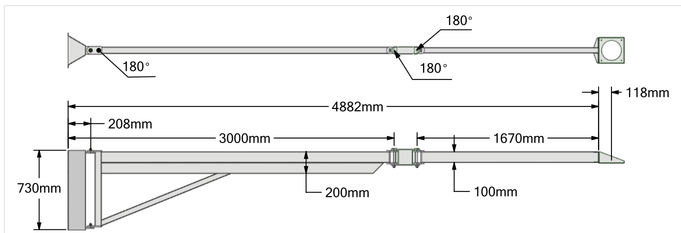
Wall console
