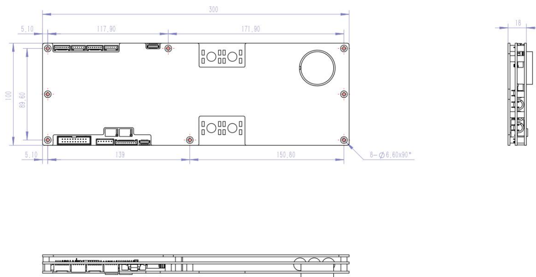
JK-PB1/2A16S-10/15/20P 外形尺寸 Dimensions of JK-PB1/2A16S-10/15/20P
