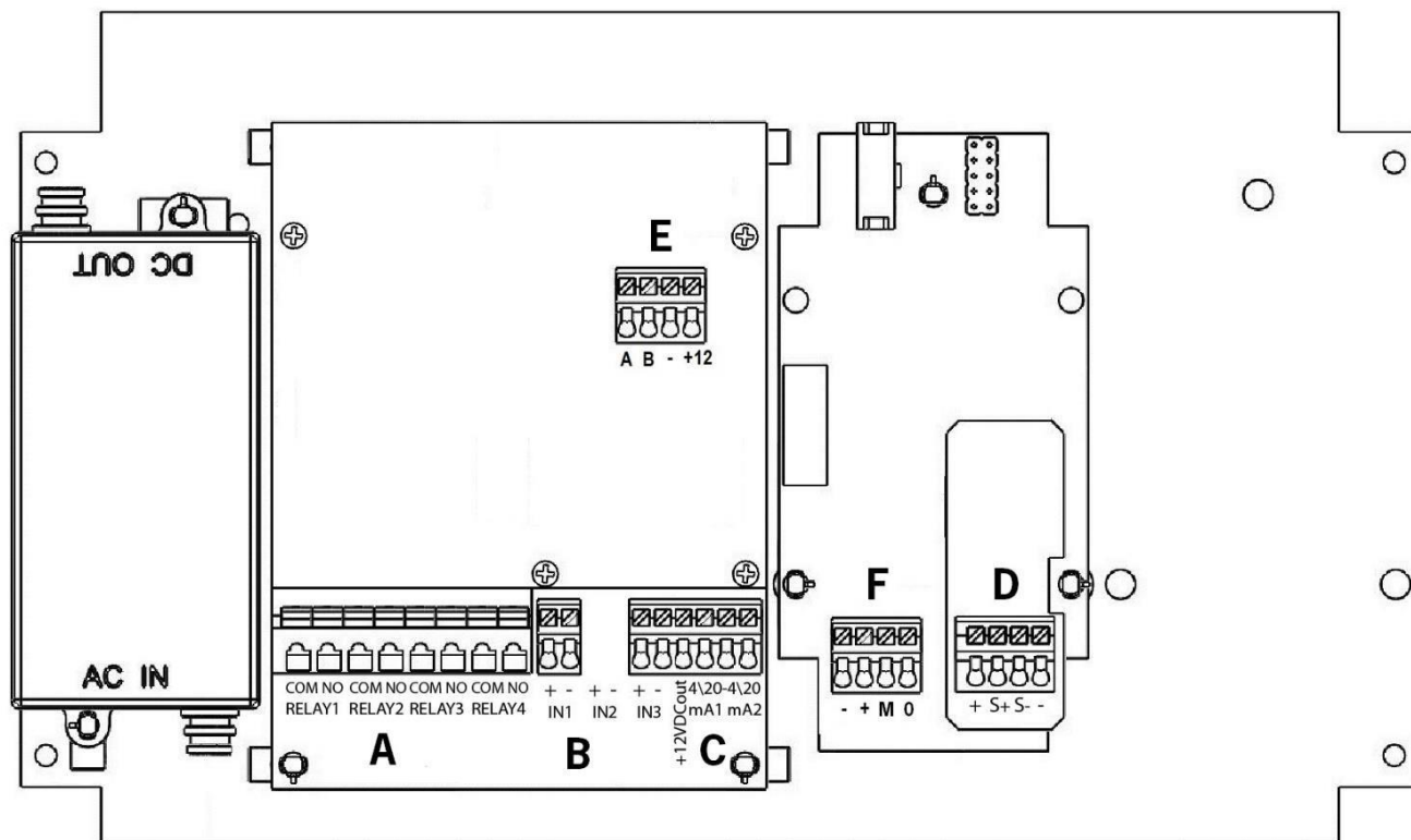
Fig. 3 – Connection diagram
