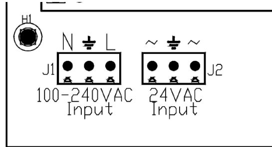
Fig. 1 – Electrical connection
