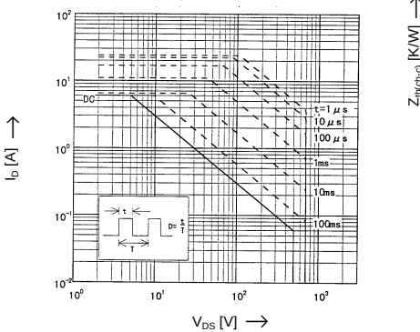
Safe operation area
