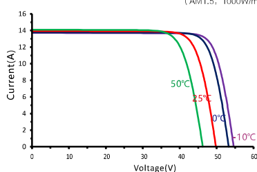
I-V characteristics at different temperatures (AM1.5, 1000W/m 2 )
