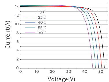
Current-Voltage Curve JAM72D40-570/GB
