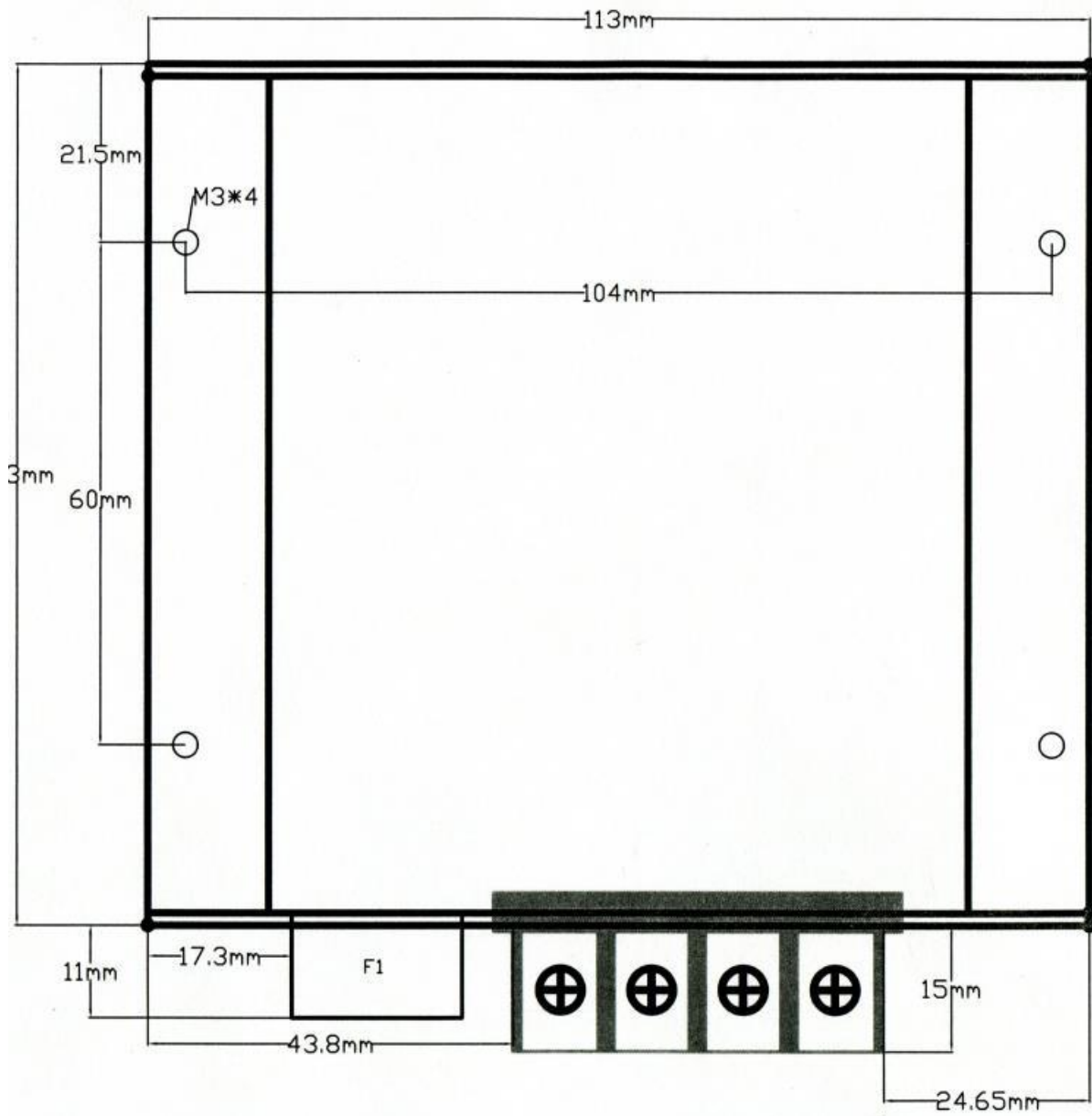
100*113*35mm shell installation dimension drawing
