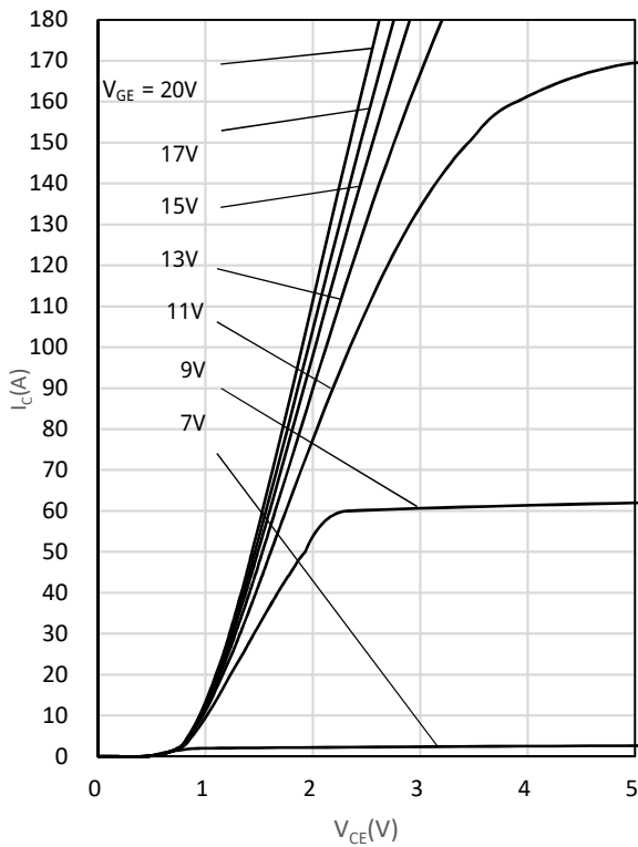
Fig. 1 Output characteristics
