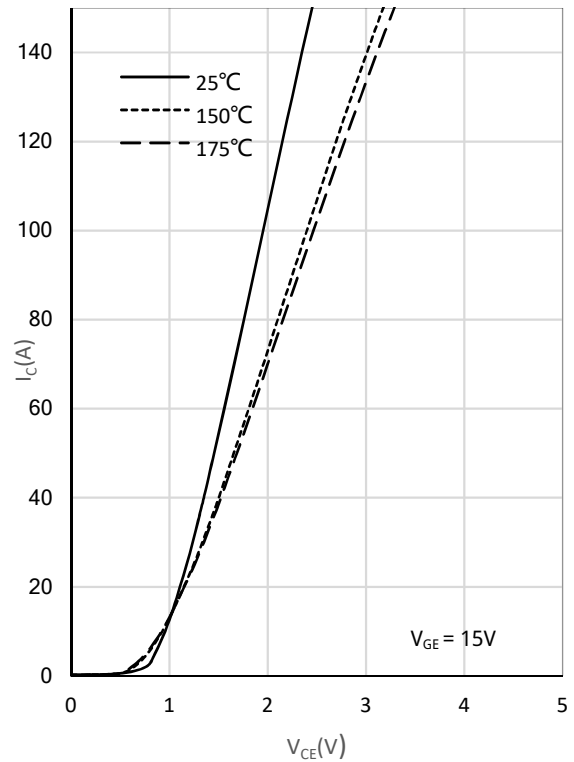
Fig. 2 Saturation voltage characteristics
