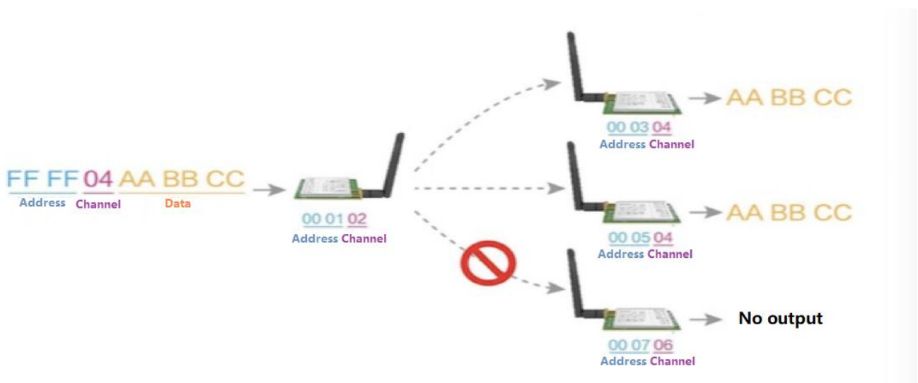
Figure 5-2 Broadcasting Transmission
