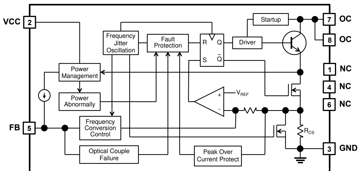
Figure.1 Functional block diagram of CSC7203
