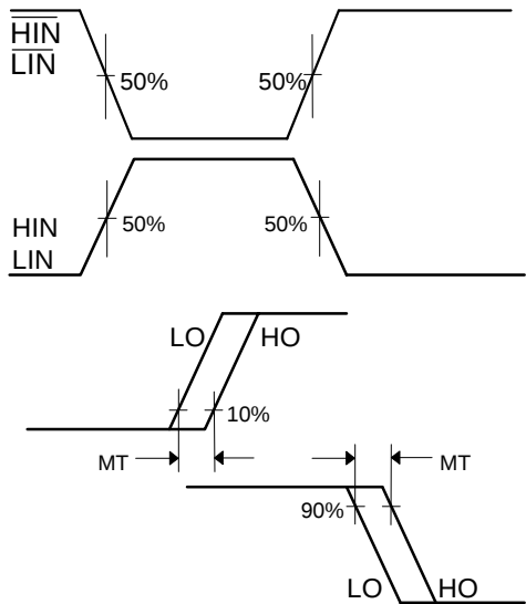
Figure 3. Delay Matching Waveform Definitions
