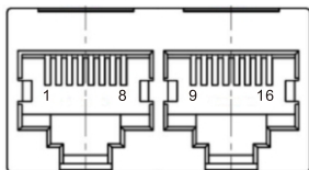
Parallel port
