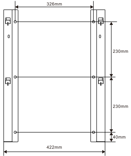
The dimensional drawing of dedicated rack for LP18PRO-48200
