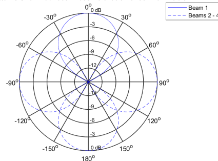
TTM-X Polar Responses at Center of Tracking Zones Patterns Shown at 4000Hz at an elevation of 30° from Table
