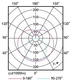
Light Distribution Diagram - Ledtube DE 1200mm 18W 765 T8 G13 RCA
