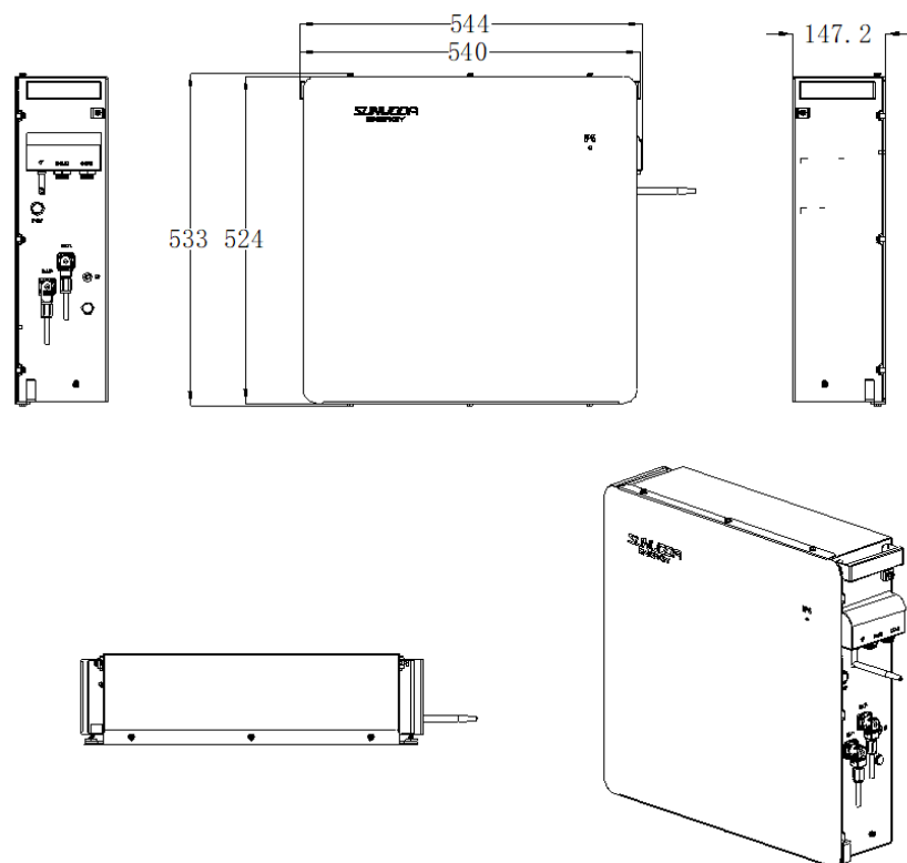
Figure 1.2-1 Dimensions of module
