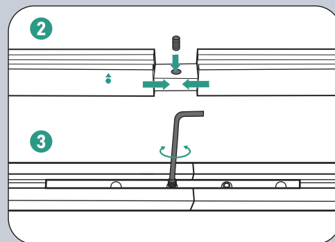
2. Putting the screws in the holes then assemble light bar.
