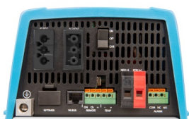
MultiPlus 500 / 800 / 1200 / 1600 BA
