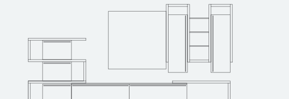
COMP. SA1346 L. 3500 x P. 250/361/490 x H 1860 mm
