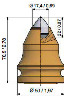
■ BKH110 BS38H-17.5070A
