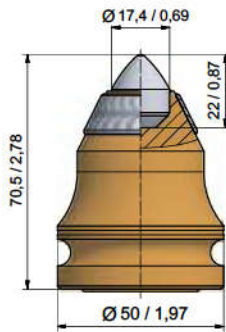
■ BKH110P BS38H-17.5070AP
