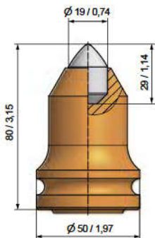
■ BKH41 B47K19LK80-H
