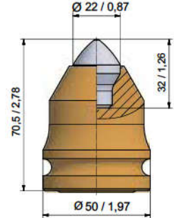
■ BKH130 BS38H-70.5070
