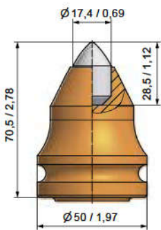
■ BKH80 B47K17.5LK70-H
