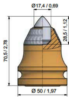
■ BKH80P B47K17.5LK70-HP
