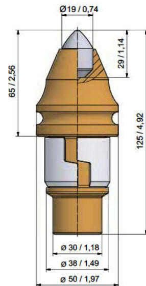
■ BKH40 BS38H-19.5065
