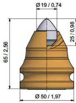
■ BKH83 BS38H-19.5065
