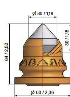
■ BKH92 BS38H-30.6064
