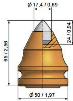
■ BKH140 B47K17.5-H/2
