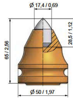
■ BKH28 BS38H-17.5065
