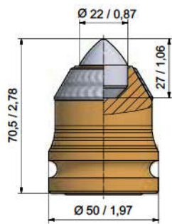
■ BKH105P BS38H-22.5070P
