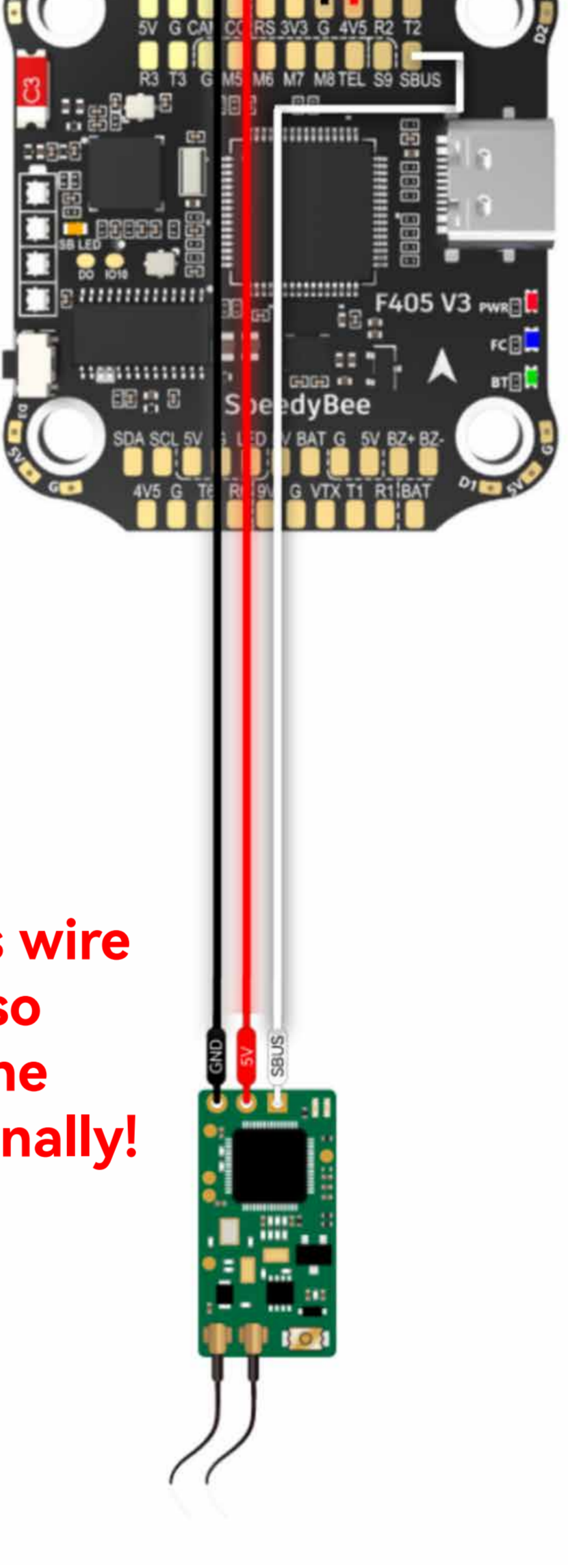
SBUS Receiver
