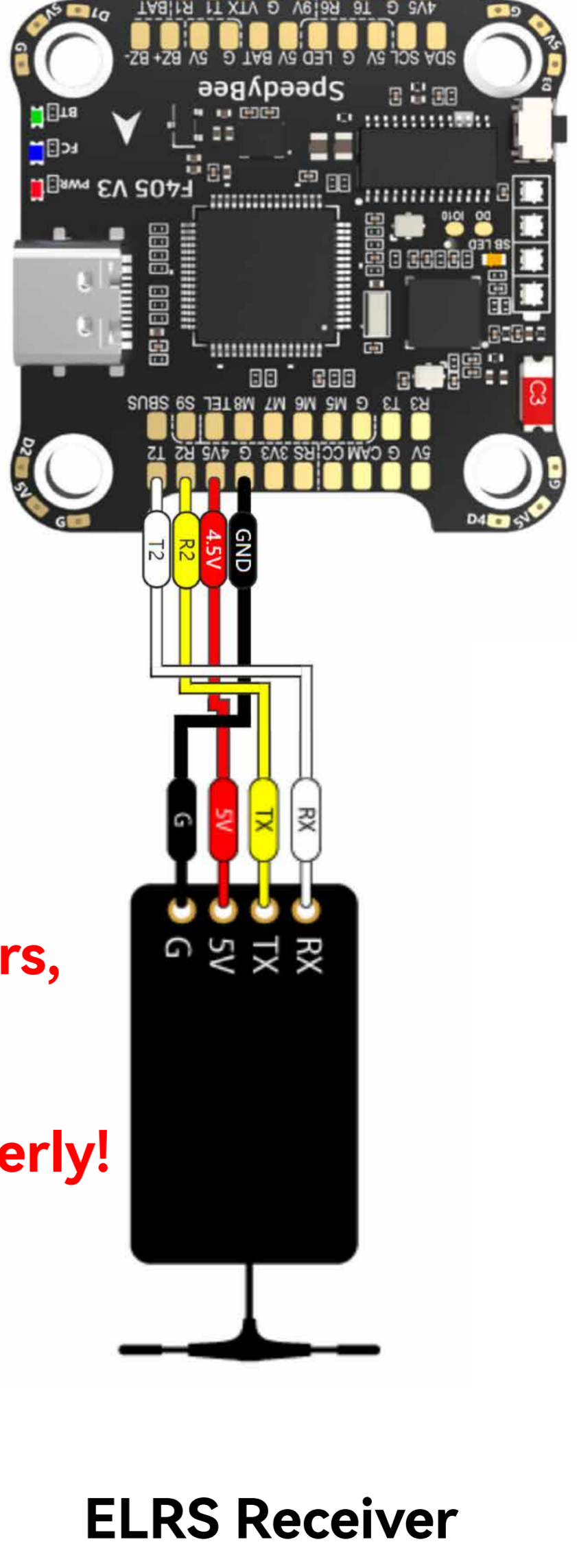
ELRS Receiver
