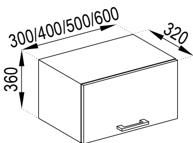
A 30/40/50/60 (320) HC 30/40/50/60 (320)
