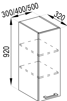
B 30/40/50 (920) U 30/40/50 (920)
