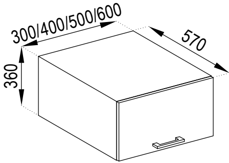
A 30/40/50/60 (570) HC 30/40/50/60 (570)
