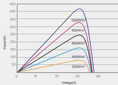
P-V CURVES OF PV MODULE(415W)
