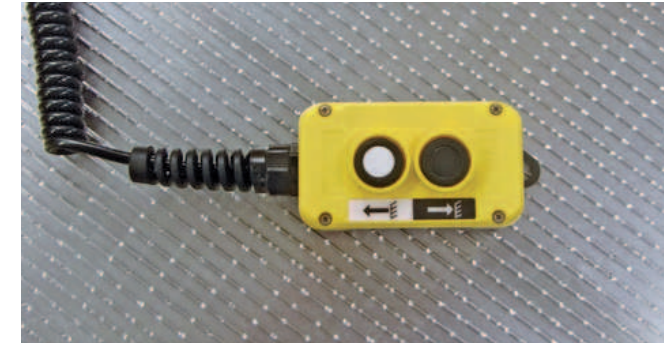
Cable remote control (option) with two functions, incl. platform marking for the assigned operating position. Socket for cable remote control pre-fitted on the control box or available for fitment inside the body.
