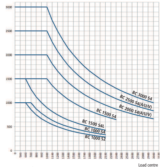
Load diagram of Standard product group
