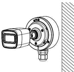
Figure 2-5 Combine the Junction Box Cover back to its Body
