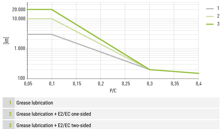
Fig. 8.25: Relubrication intervals with grease lubrication, one-sided and two-sided long-term lubrication unit (E2/EC) for HG, EG, CG, WE. The long-term lubrication unit (E2/EC) is not available for the WE series.
