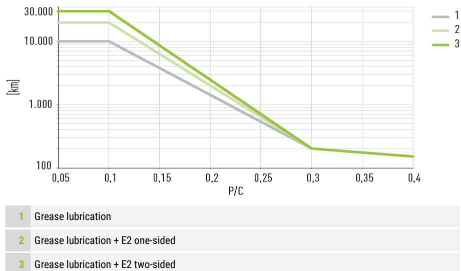
Fig. 8.26: Relubrication intervals with grease lubrication, one-sided and two-sided long-term lubrication unit (E2/EC) for QH, QE and QW. The long-term lubrication unit (E2/EC) is not available for the QW series.
