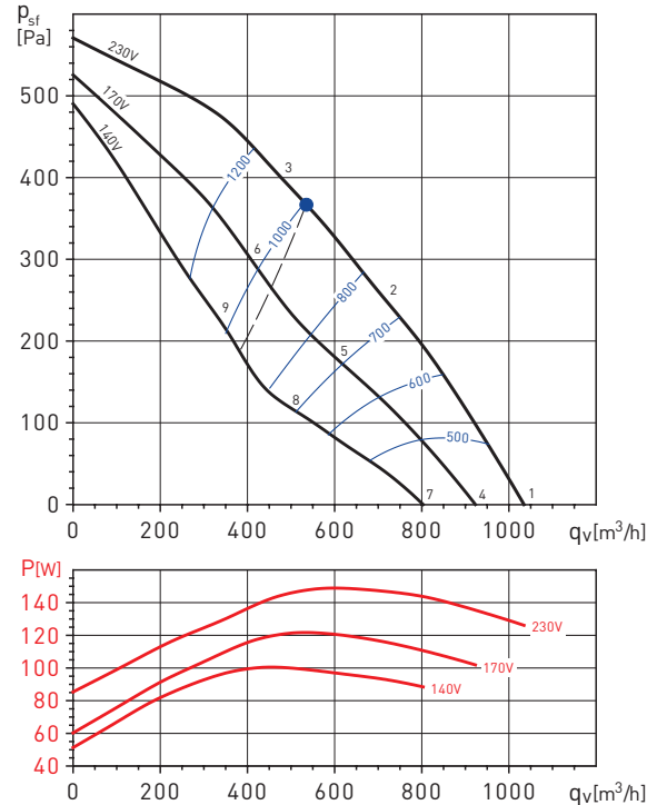
VENT-250NK
