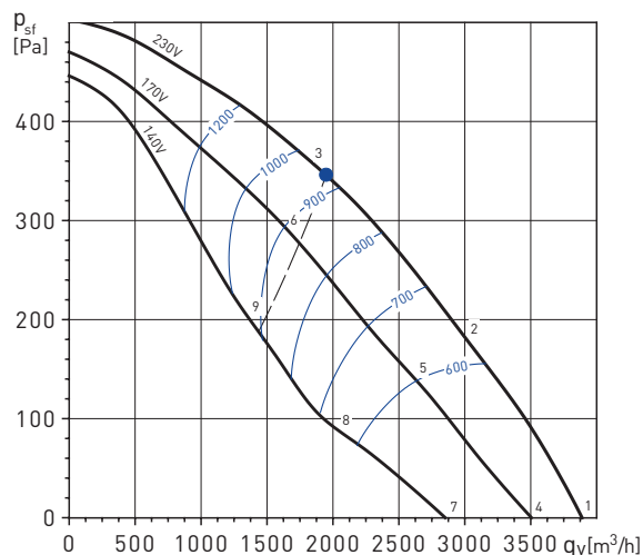
VENT-400N
