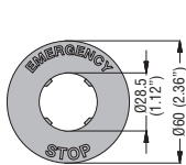
Plastic disk for mushroom-head pushbuttons
