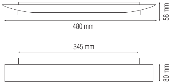
Technical Drawing
