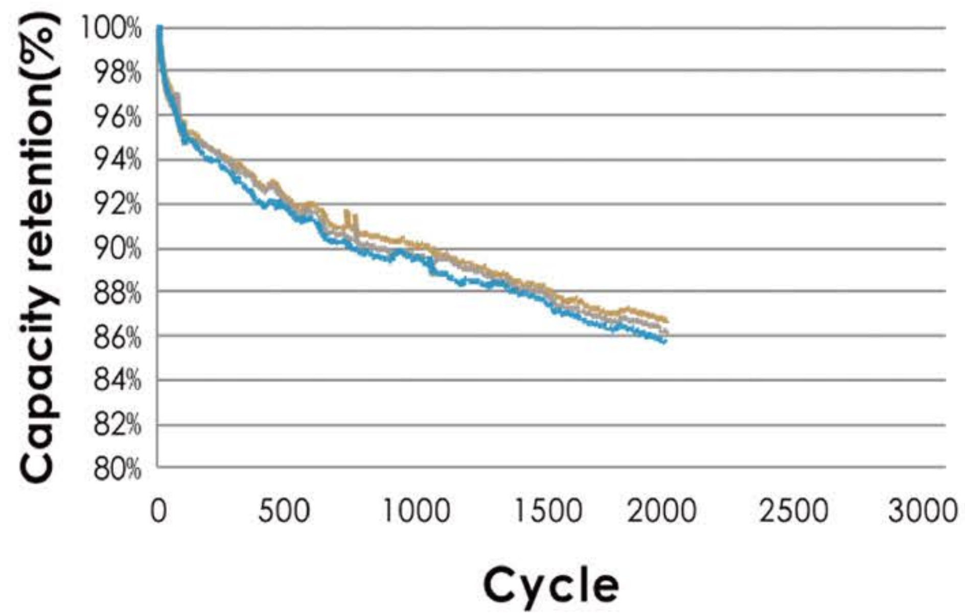
Cycle Test @ RT 1.0C/1.0C
