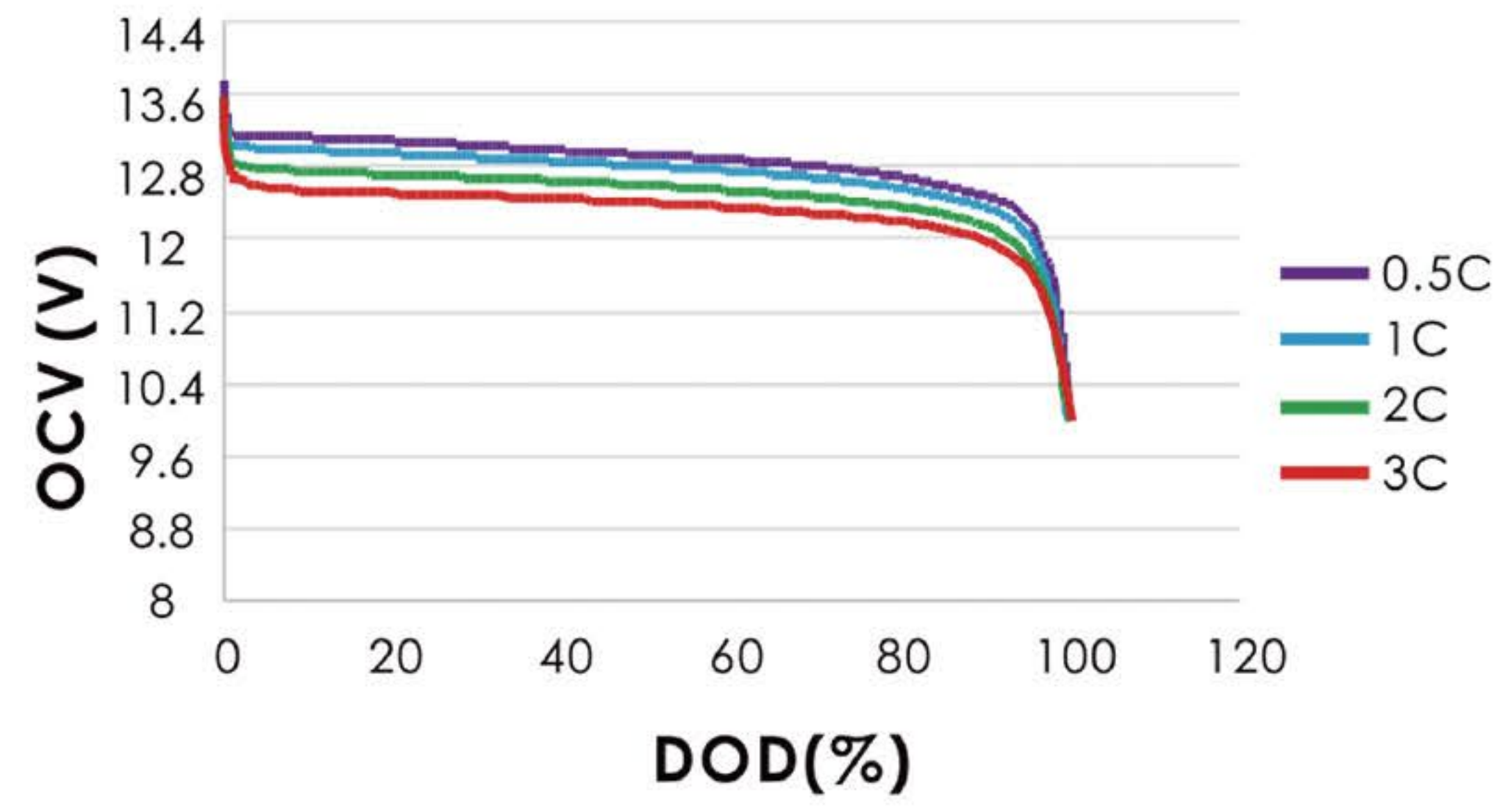
DC Rate Test
