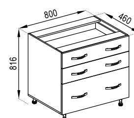
H 80 3Ш (2+1) D 80 3Dr (2+1)
