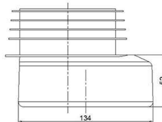
VISTA FRONTALE FRONT VIEW
