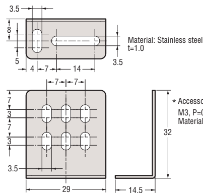
OP-66846 L-shape mounting bracket for LV-S41/LV-S41L (Option)
