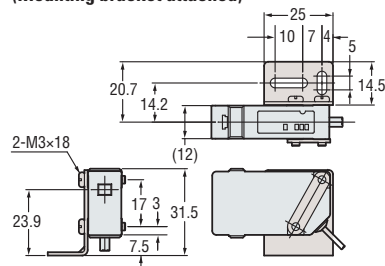
LV-H64/H65 (Mounting bracket attached)
