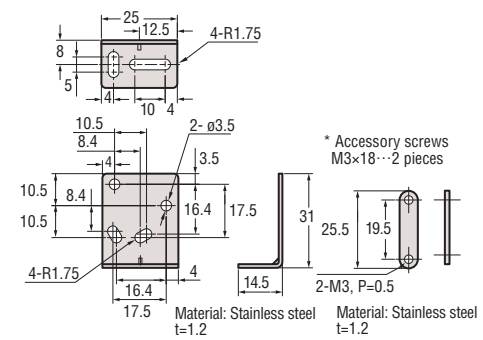
Mounting bracket (Accessory)
