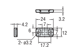
Reflector R-7 for LV-H62 (Accessory)
