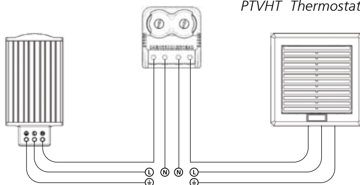
PTVHT Thermostat Wiring Diagram
