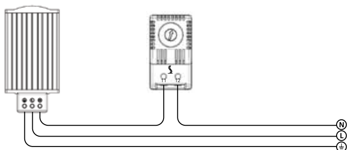
PTHT Thermostat Wiring Diagram
