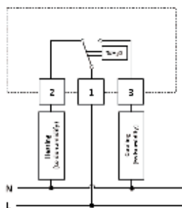
PHG02 Hygrostat Wiring Diagram
