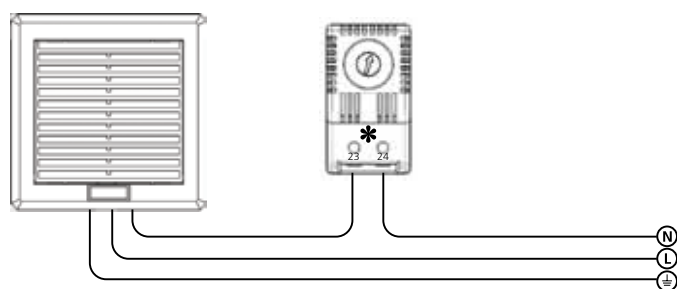
PTVT Thermostat Wiring Diagram
