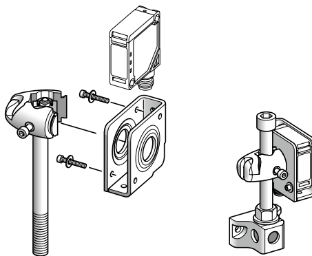
Mounting example
