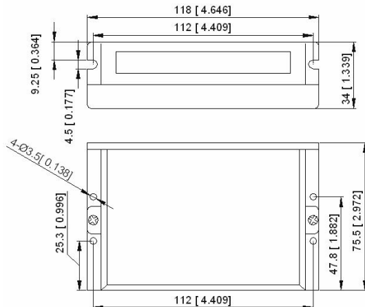
Figure 1: Installation specifications
